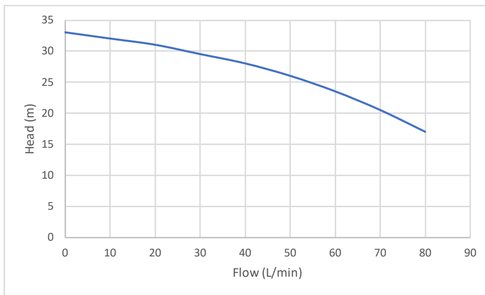
Figure 2 Pedrollo NK 2/2-N characteristic curve (power 0.37 kW)
