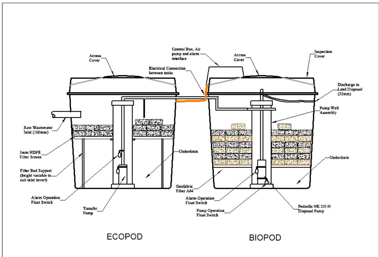
Figure 1 Biolytix MultiPod wastewater treatment system
